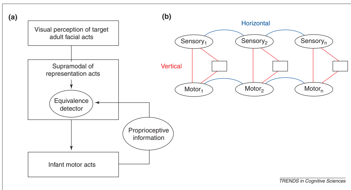
Fig. 1. Theories of imitation that address the problem of perceptual opacity. Schematic representations of (a) Active Intermodal Mapping (AIM) theory 18 , and (b) Associative Sequence Learning (ASL) theory 2 . (See text for further details.)
